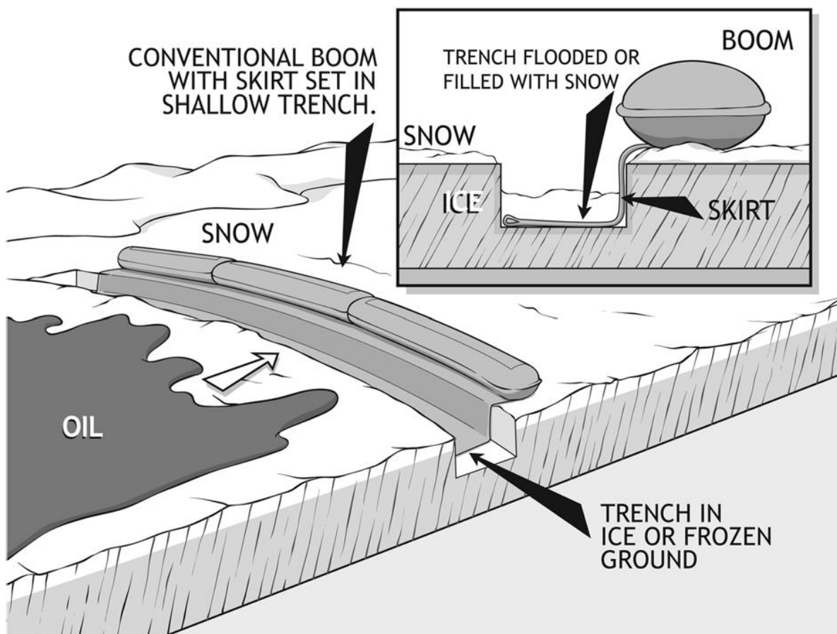
Figure 5.21 Ice Trench
