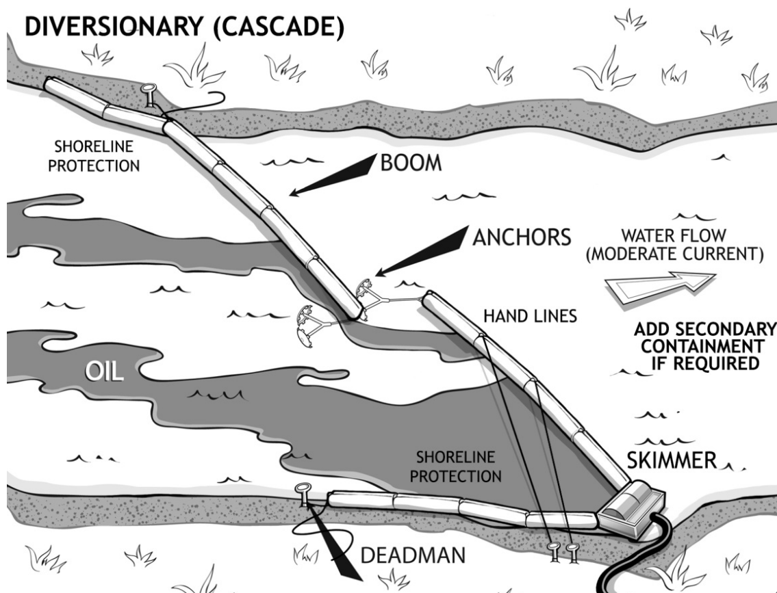
Figure 5.7 Deflection/Diversion Boom
