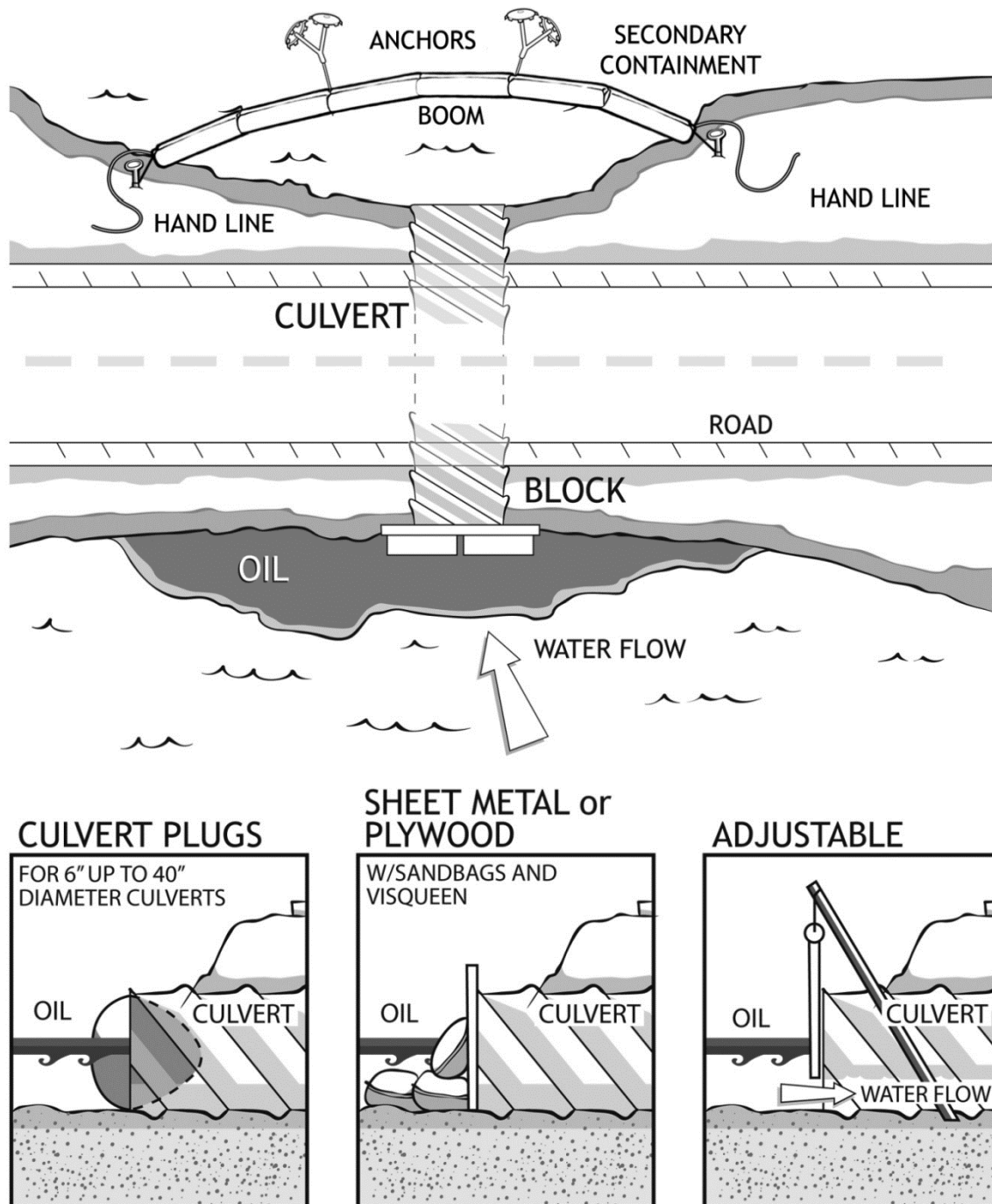
Figure 5.2 Culvert Blocking
