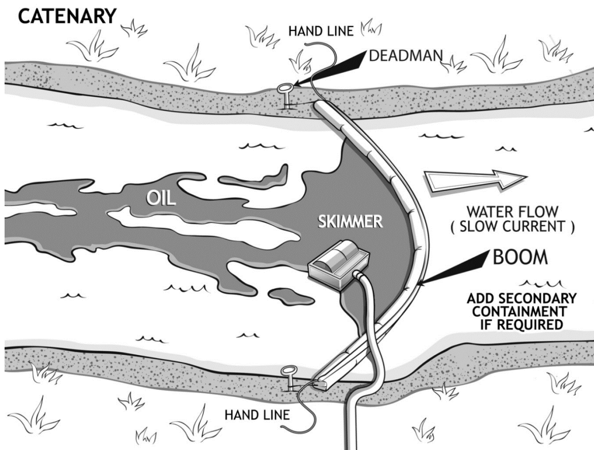
Figure 5.6 Catenary Boom
