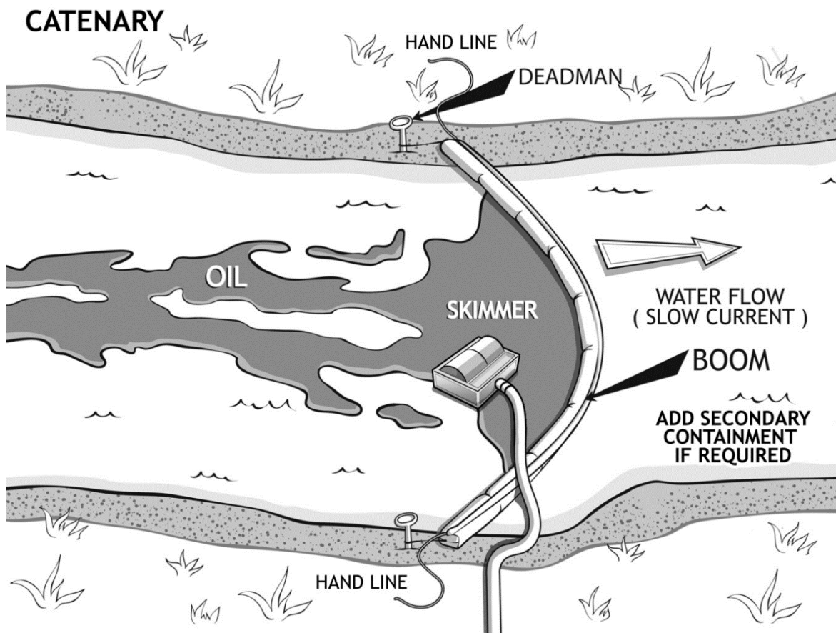
Figure 5.6 Catenary Boom
