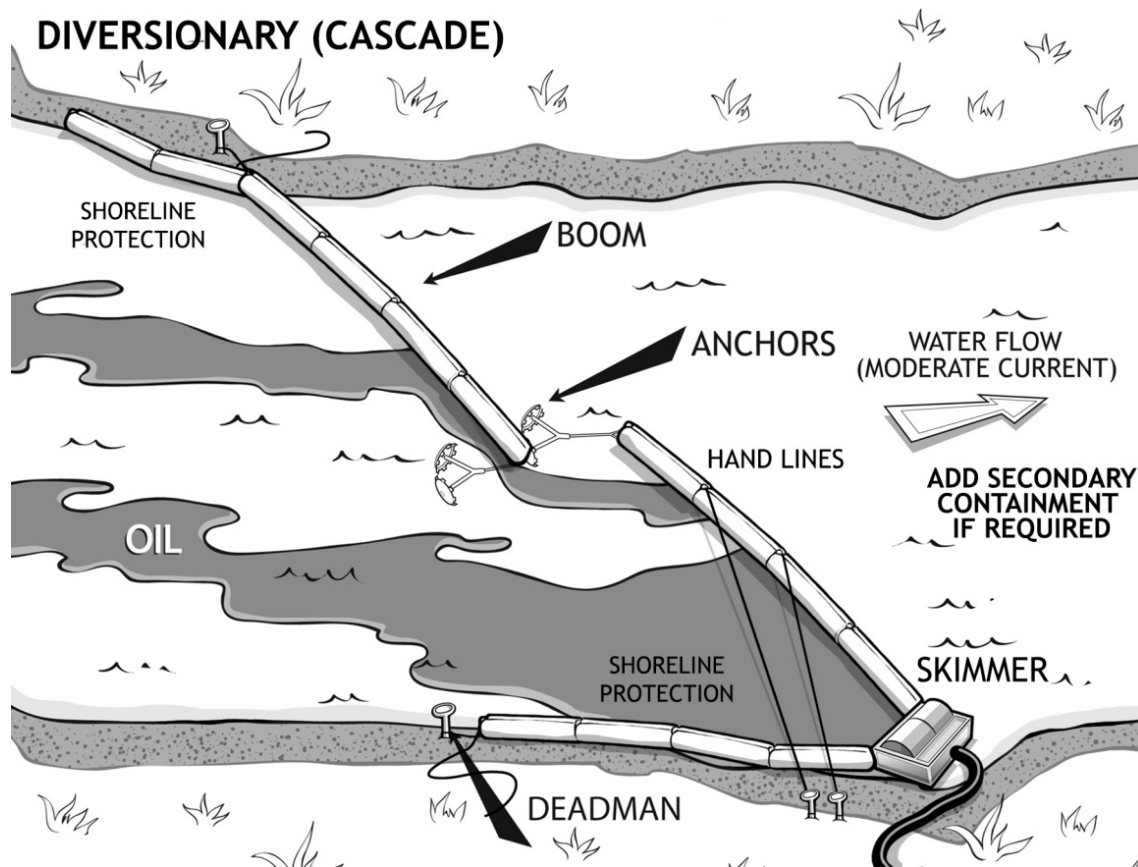
Figure 5.7 Deflection/Diversion Boom
