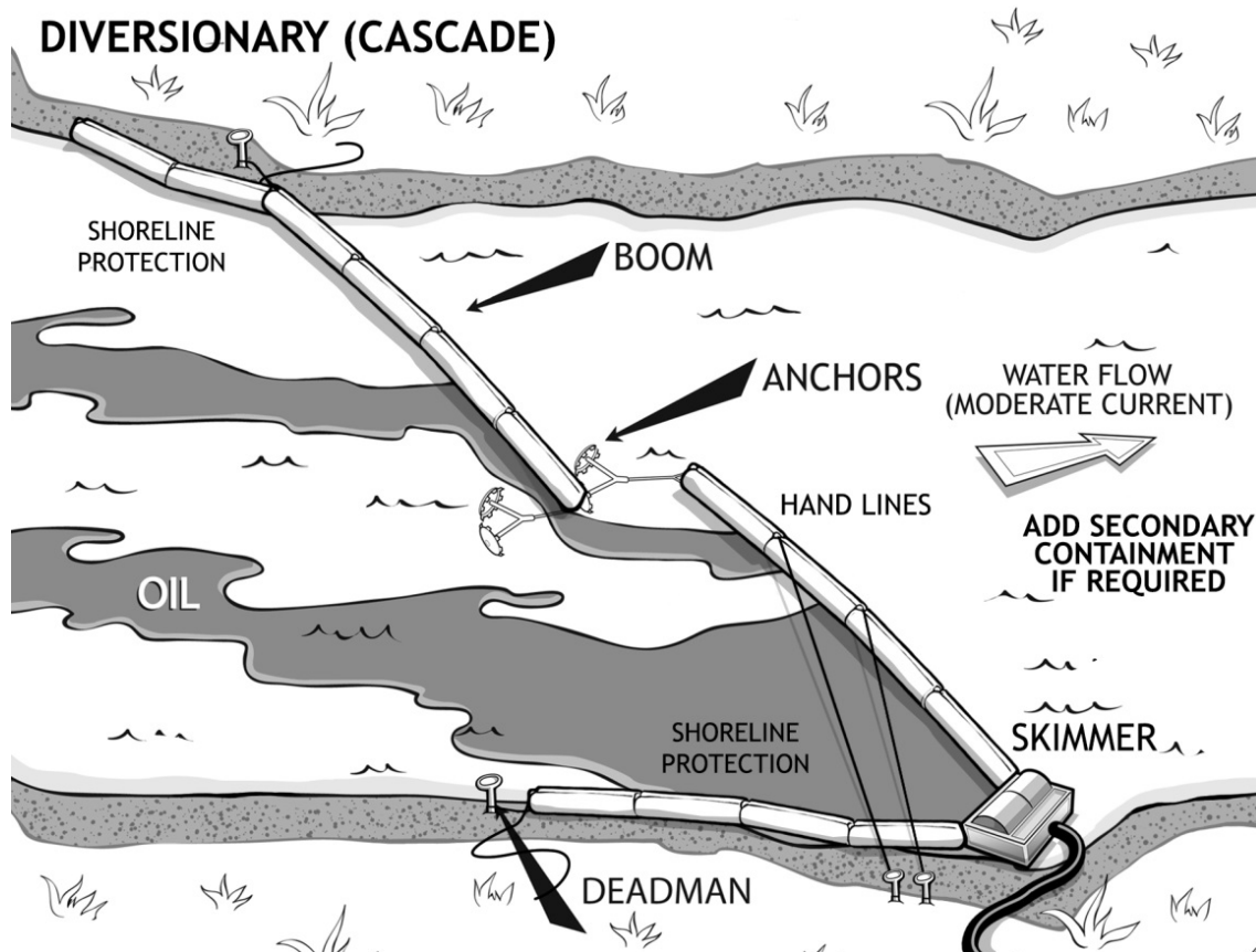
Figure 5.7 Deflection/Diversion Boom
