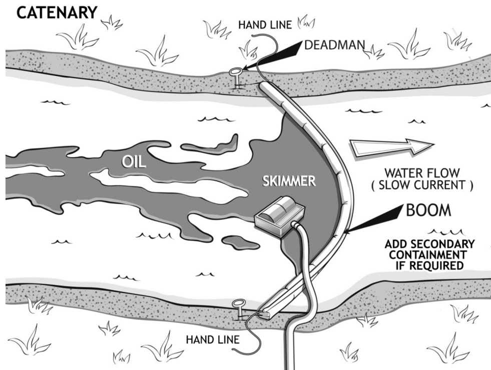
Figure 5.6 Catenary Boom
