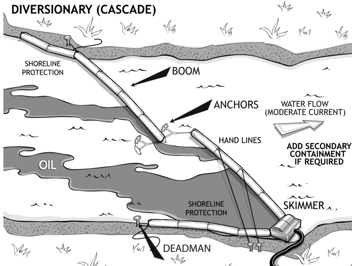
Figure 5.7 Deflection/Diversion Boom
