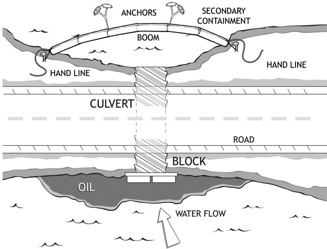
Figure 5.2 Culvert Blocking
